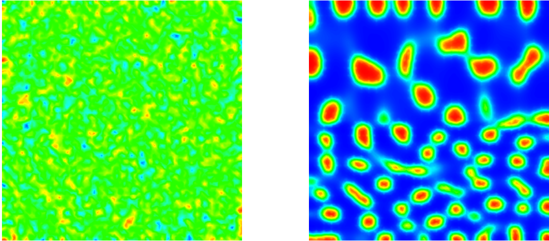
Figure 8: Pattern formation for the full chemotaxis model (2.1) on a 2-D domain \Omega = (0, 10) \times (0, 10) at time t = 0 s with 0 \leq u \leq 1 (left) and at time t = 0.5 s with 6.93^{-3} \leq u \leq 0.99 (right).
