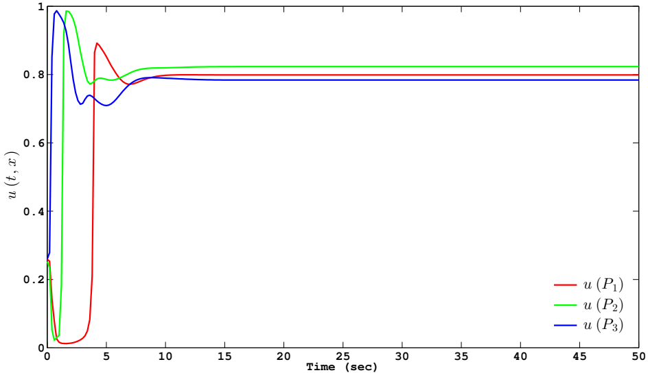
Figure 4: The evolution of the cell density with respect to the time at three different points: P_1(5.25; 6) in the red line, P_2(5; 1.25) in the green line, P_3(4.35; 8.1) in the blue line.
