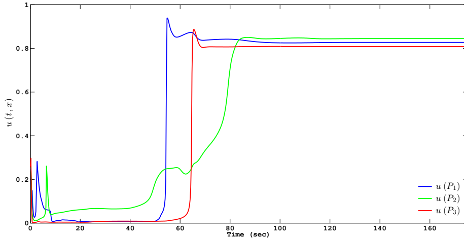
Figure 10: The evolution of the cell density with respect to the time at three different points: P_1 (5.70; 4.05) in the blue line, P_2 (3.28; 6.88) in the green line, P_3 (2.80; 3.75) in the red line.
