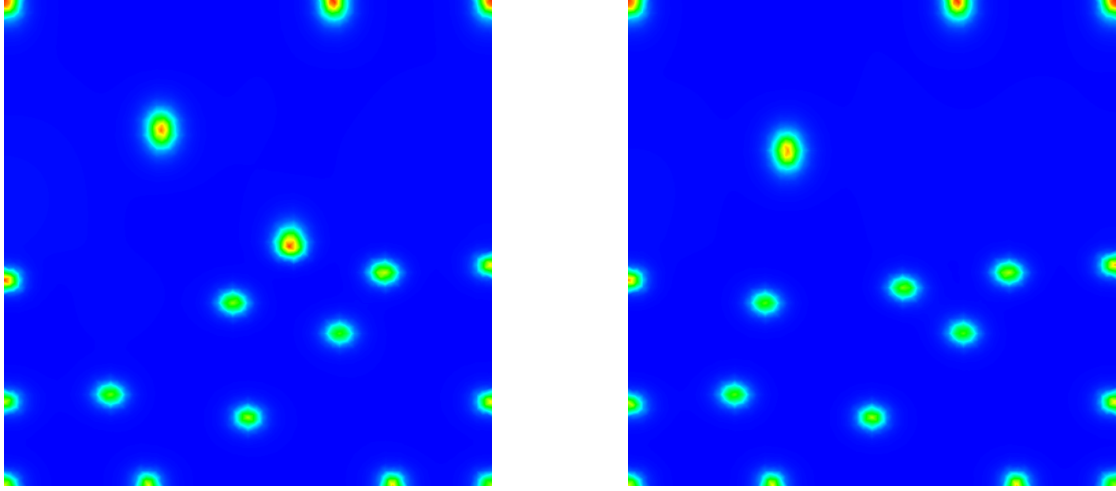
Figure 9: Pattern formation for the full chemotaxis model (2.1) at time t = 2.35\text{s} with 3.2 \times 3.67^{-3} \leq u \leq 0.88 ( left ) and at time t = 40\text{s} with 4 \times 4.3^{-3} \leq u \leq 0.8447 ( right ).
