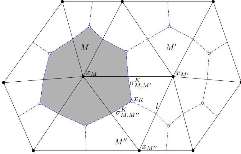
Figure 1: Donald dual mesh; control volumes, centers, interfaces.
