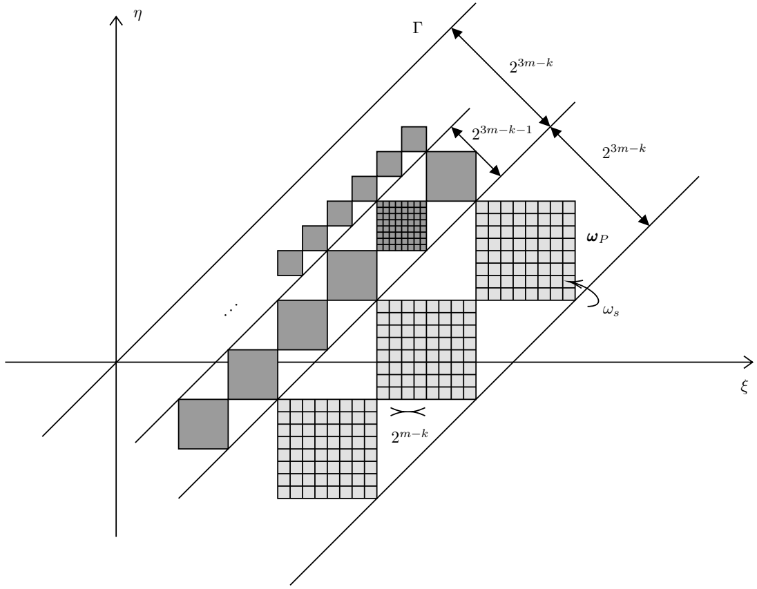
FIGURE 1. Geometry in the frequency plane of squares \omega_s, \omega_P for m = \frac{3}{2}
