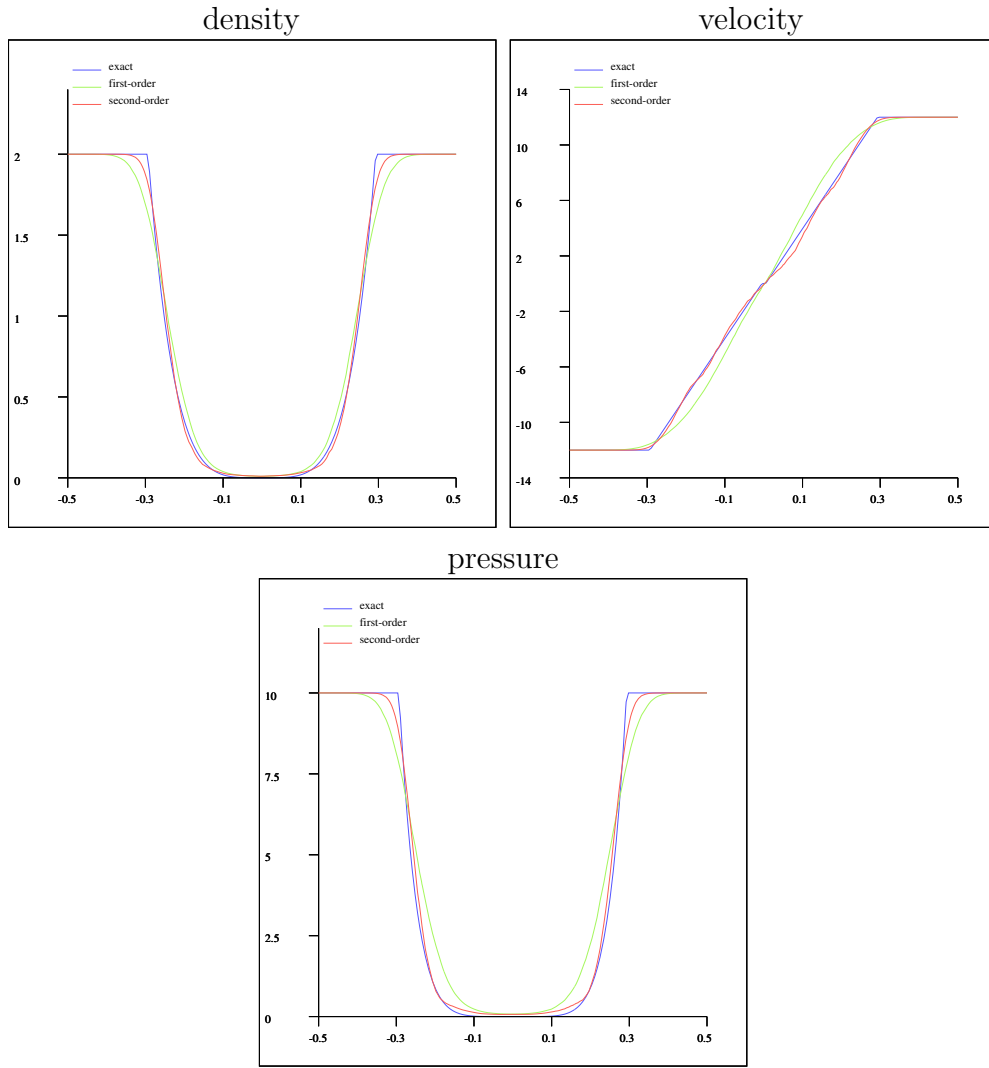
Fig. 6. Double rarefaction waves. Comparison of the exact solution and both first-order and second-order approximate solution.
