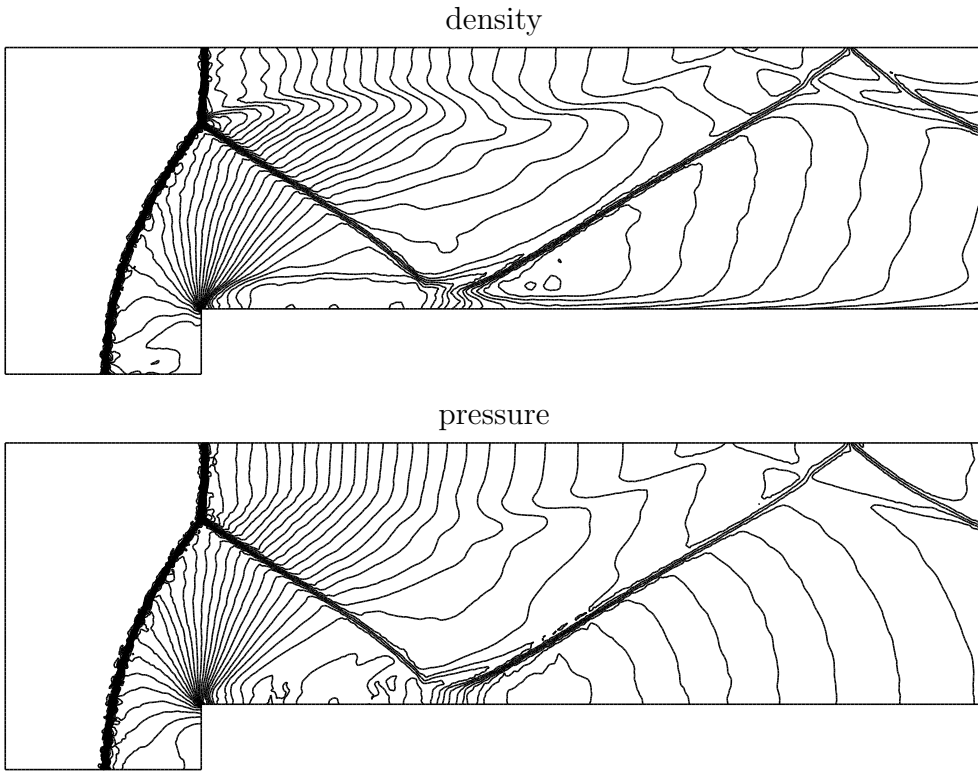
Fig. 8. Mach 3 wind tunnel with a step. Density and pressure at time t = 4 , 30 isovalues from 0.7 to 6.5 for the density and from 0.5 to 11.9 for the pressure.
