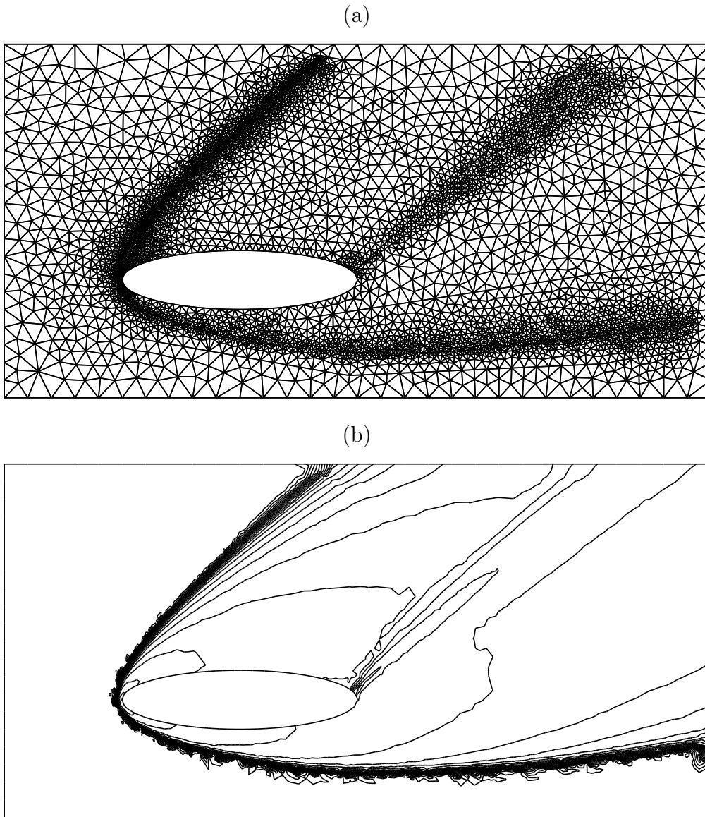
Fig. 9. Ellipse at 25 Mach number. (a) Adapted grid made of 4810 nodes and 9421 triangles. (b) Mach number with 30 isovalues from -0.2 to 29 .
