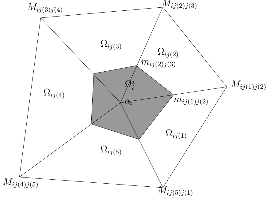
Fig. 2. Sub-cell decomposition of the dual-cell \Omega_i
