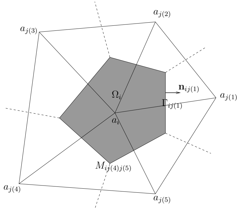
Fig. 1. Cell-center control volume: dual cell \Omega_i
