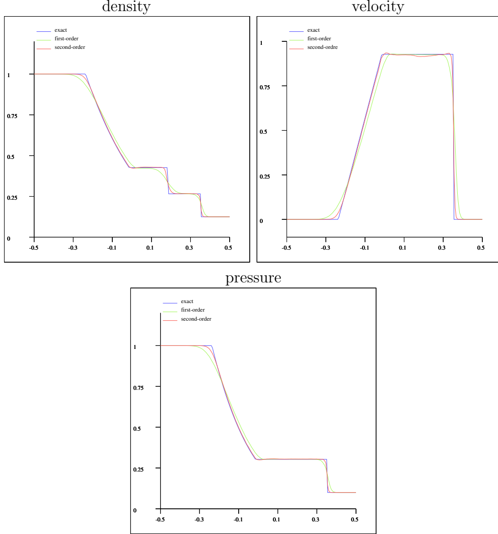
Fig. 5. Shock tube. Comparison of the exact solution and both first-order and second-order approximate solution.
