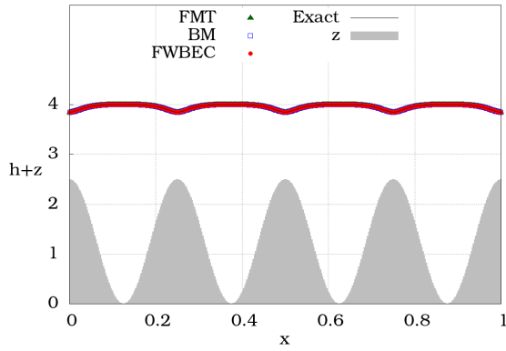
FIGURE 6. On the left: numerical results at time 1.0 for the steady state problem (95) with the legend FWBEC: fully well-balanced entropy satisfying solver given by Theorem 6.1, BM: scheme derived in [15] associated to the Rusanov numerical flux [45], FMT: scheme derived in [22, Section 3.2]. On the right: errors between the exact and the numerical solutions at time 1.0 for the variables h, hu .
