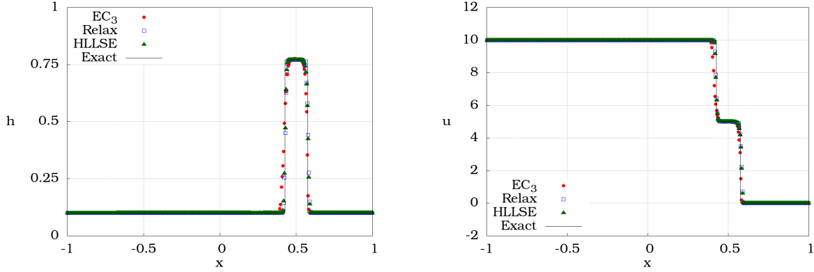
FIGURE 2. Numerical results at time 0.1 for the initial condition (89), with the legend EC_3 : Lemma's 4.2 solvers, Relax: Suliciu relaxation and HLLSE: solver [30, Section b.ii].
