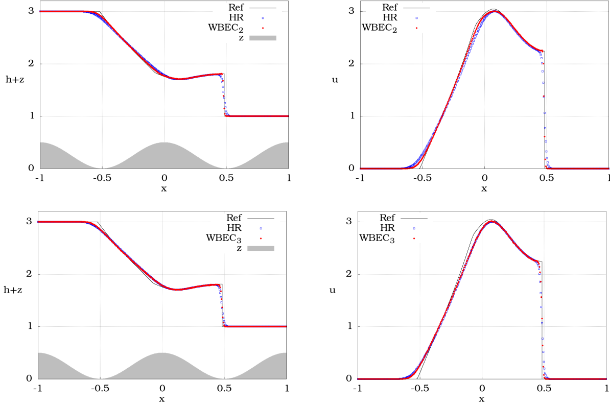
FIGURE 5. Numerical results at time 0.1 for the dam break problem (92) on a mesh composed of 400 cells with the legend (WBEC_i)_{i \in \{1, \dots, 3\}} : Theorem 5.1 solvers with the configurations (93), HR: hydro-static reconstruction [3] with the Rusanov numerical flux [45].
