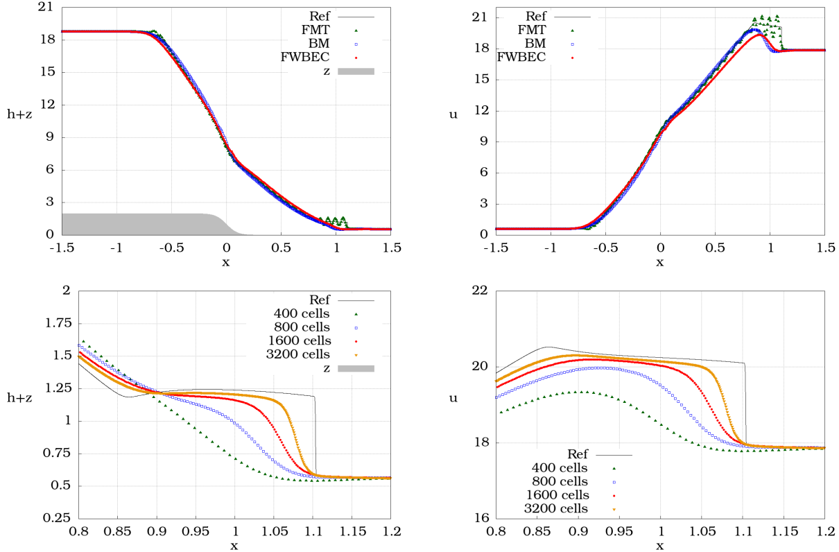
FIGURE 10. Numerical results at time 0.05 on a mesh composed of 400 cells for the problem (96) with the legend FWBEC: Theorem 6.1 solver, BM: scheme derived in [15] associated with the Rusanov numerical flux [45], FMT: scheme derived in [22, Section 3.2]. At the bottom, numerical results with a mesh refinement for the FWBEC scheme. For the clarity, the display is zoomed in on the shock wave near x = 1.1 .
