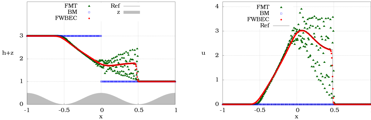
FIGURE 9. Numerical results at time 0.1 on a mesh composed of 400 cells for the dam break problem (92) with the legend FWBEC: Theorem 6.1 solver, BM: scheme derived in [15] associated with the Rusanov numerical flux [45], FMT: scheme derived in [22, Section 3.2].
