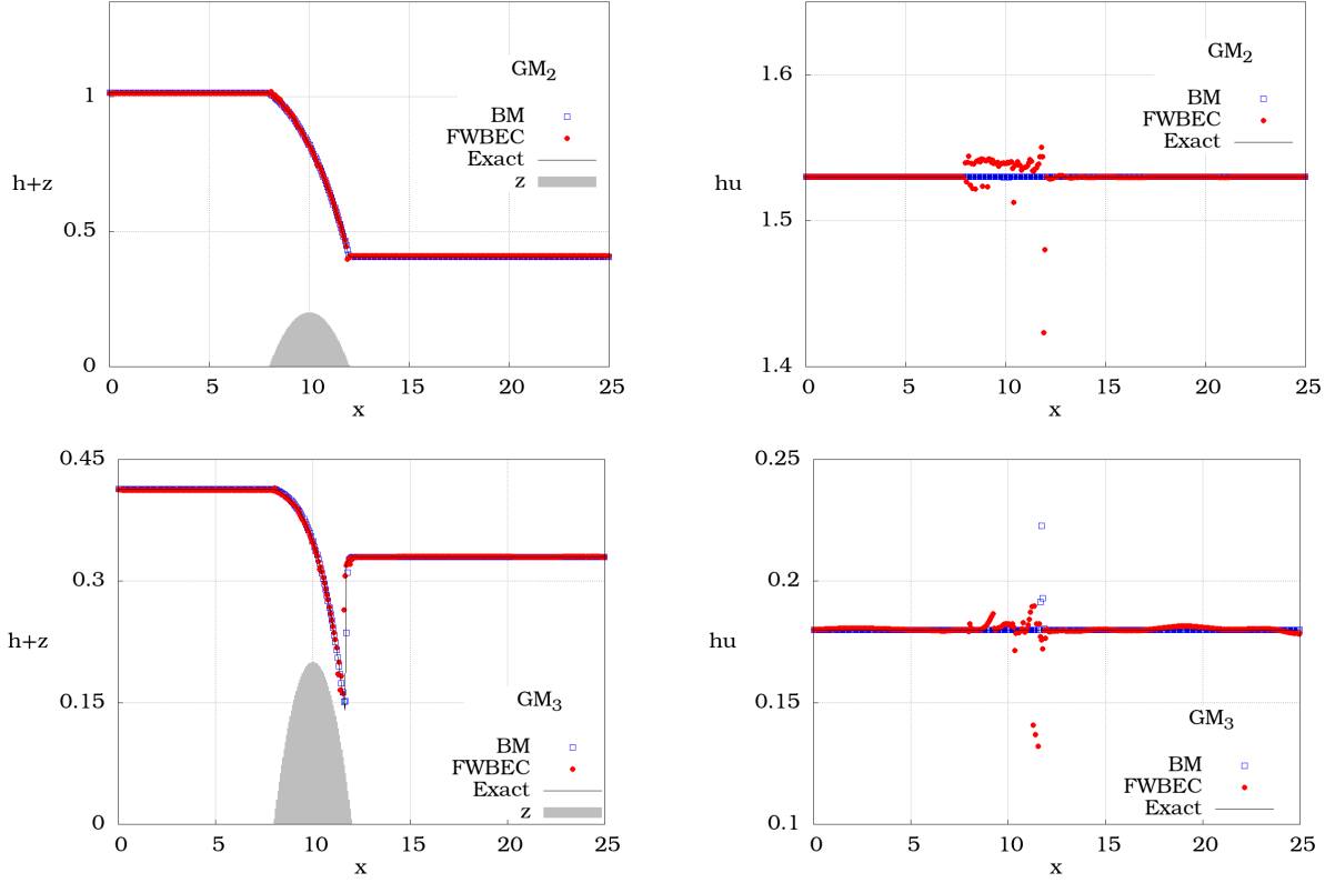
FIGURE 7. Numerical results for the Goutal and Maurel's problems (91) on a mesh composed of 400 cells. The legend is FWBEC: fully well-balanced entropy satisfying solver given by Theorem 6.1, BM: scheme derived in [15] associated to the Rusanov numerical flux [45].
