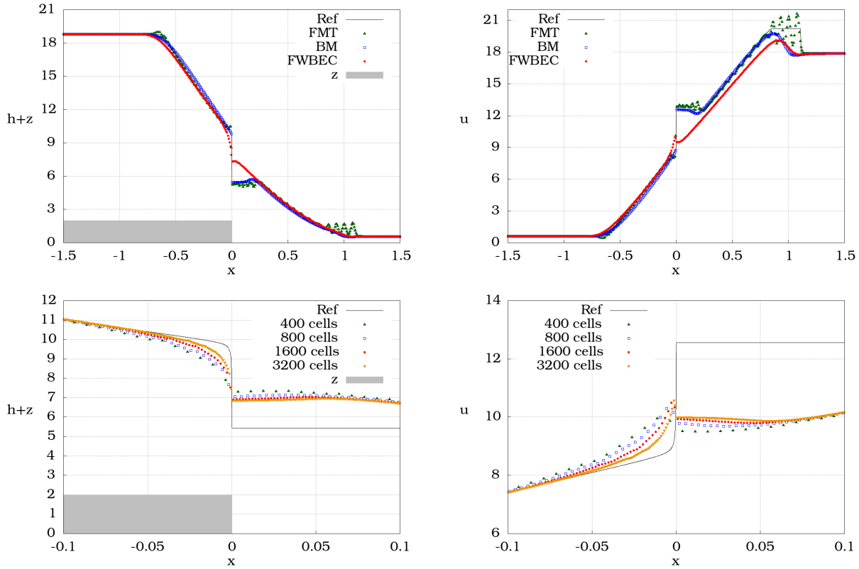
FIGURE 11. Numerical results at time 0.05 on a mesh composed of 400 cells for the problem (97) with the legend FWBEC: Theorem 6.1 solver, BM: scheme derived in [15] associated with the Rusanov numerical flux [45], FMT: scheme derived in [22, Section 3.2]. At the bottom, numerical results with a mesh refinement for the FWBEC scheme. For the clarity, the display is zoomed in on the discontinuity near x = 0 .
