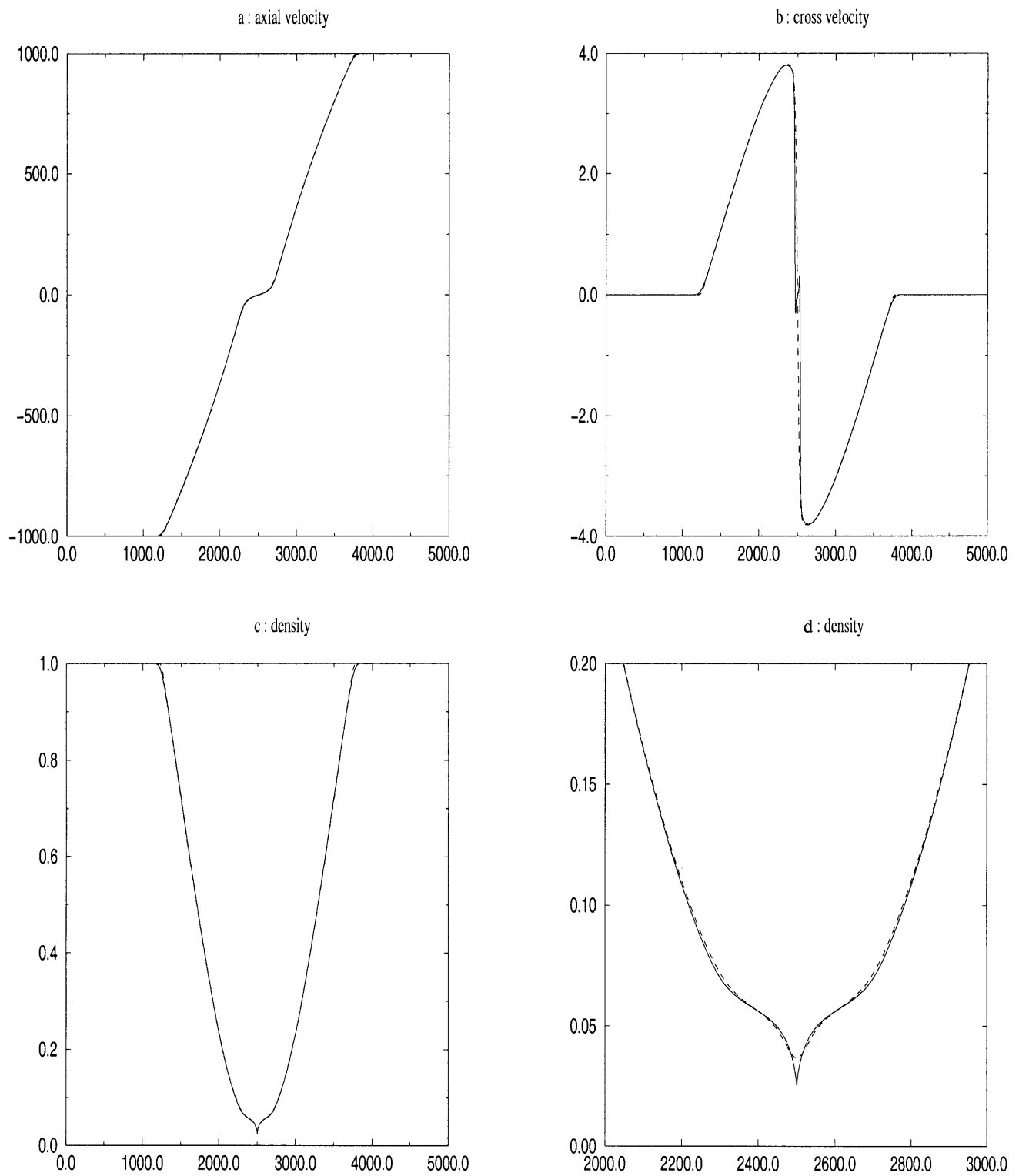
Fig. 5a–h. The third test case: a double rarefaction wave. Results for the Rusanov ( a–f – dashed lines and g ) and VFRoe ( a–f – solid lines and h ) schemes. Dashed and solid lines in g and h correspond to the Riemann invariants V_+ and V_- , respectively
