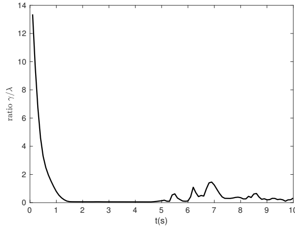
Fig. 5.15: Time evolution of the maximum ratio \gamma/\lambda .
