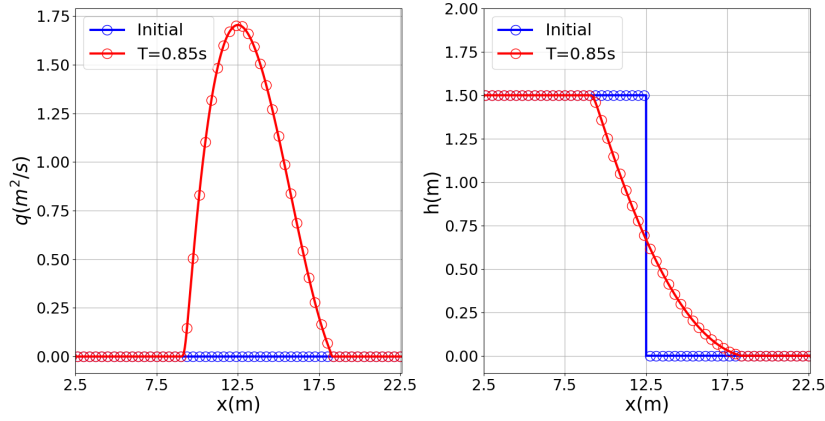
Fig. 5.7: Velocity and water height profiles at time T = 0.8s for the dam break problem with dry front.
