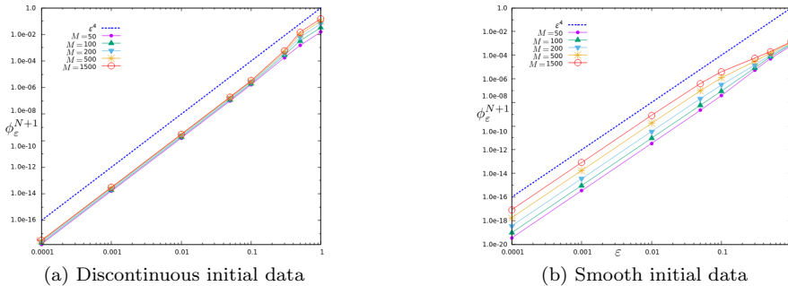
FIG. 5.1. Space integral of the relative entropy \phi_\varepsilon^{N+1} with respect to \varepsilon in log scale with C_{CFL}=0.4 and \gamma=1.4 .
