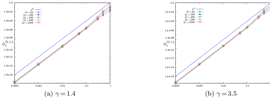
FIG. 5.3. Space integral of the relative entropy \phi_\varepsilon^{N+1} with respect to \varepsilon in log scale with the discontinuous initial data and C_{CFL}=0.4 .
