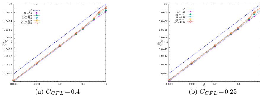
FIG. 5.2. Space integral of the relative entropy \phi_\varepsilon^{N+1} with respect to \varepsilon in log scale with the discontinuous initial data and \gamma=1.4 .
