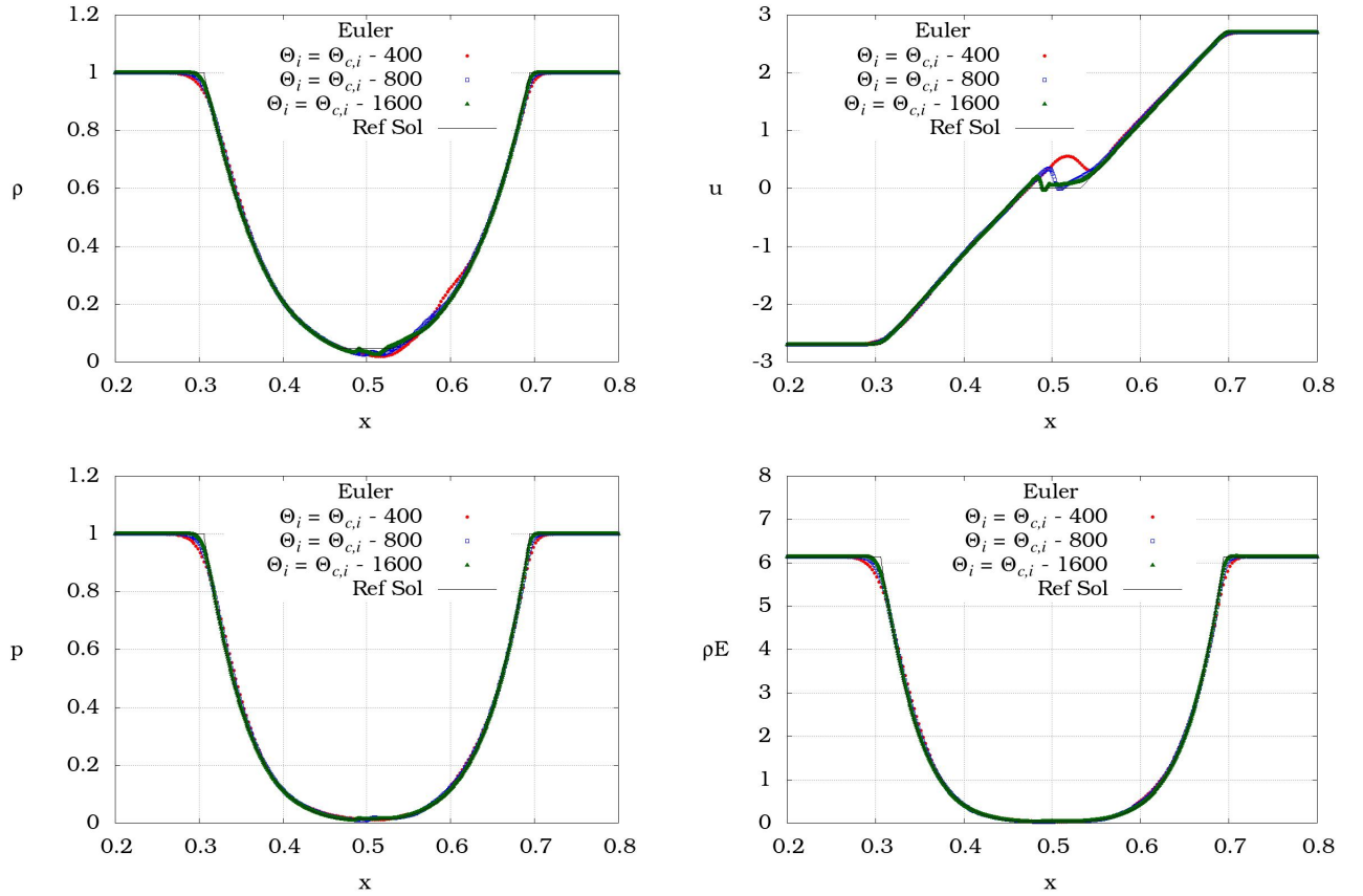
FIGURE 6. Second-order accurate approximation of the Euler solution for the double rarefaction waves problem at time t = 0.05 with a refined mesh made of 400 cells to 1600 cells.
