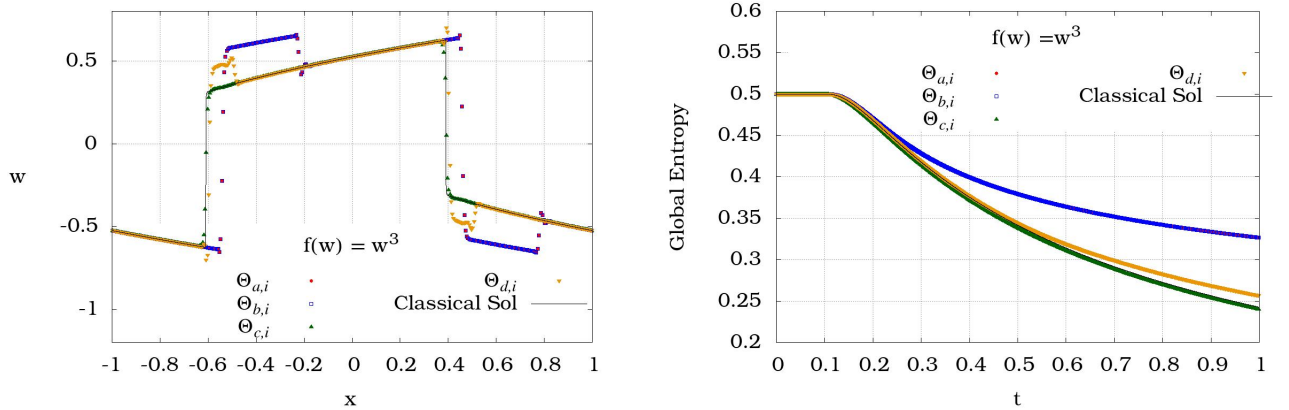
FIGURE 7. Second-order accurate approximation of the scalar conservation law with non convex flux ( f(w) = w^3 ) solution at time t = 1 with a mesh made of 400 cells: on the left non classical wave profiles, on the right the decrease of the global entropy integrated over the grid.
