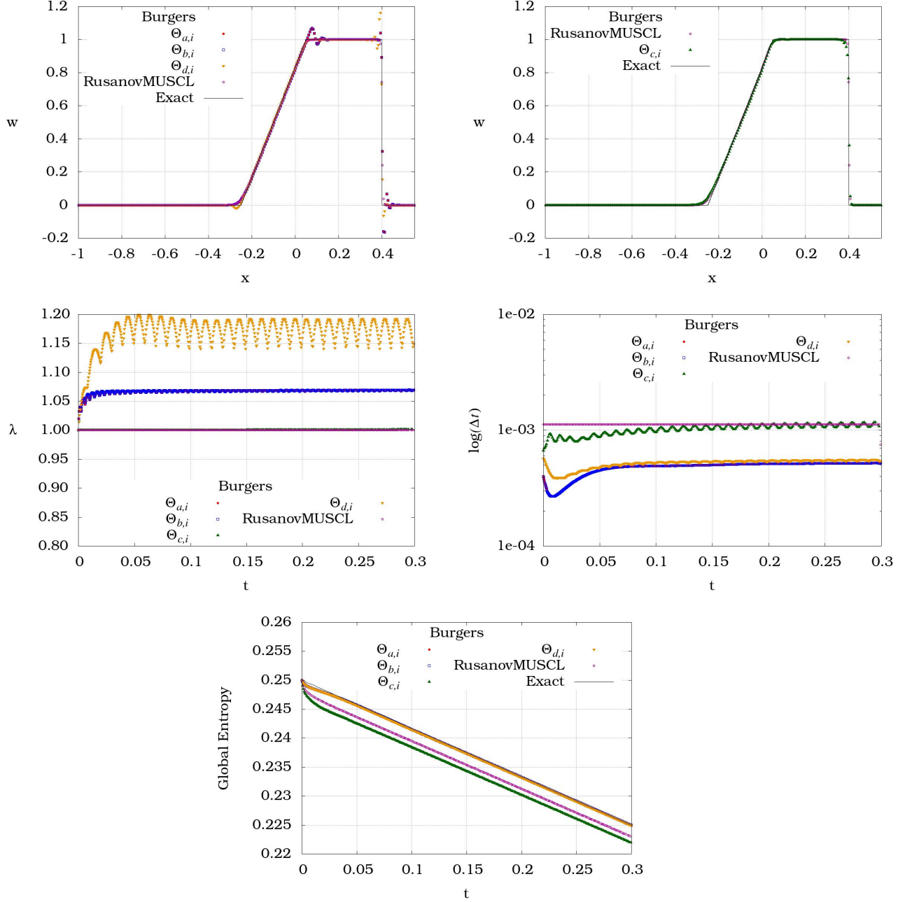
FIGURE 2. On the top, second-order accurate approximations of the Burgers solution made of rarefaction and shock waves at time t = 0.3 with a mesh made of 400 cells with periodic boundary conditions. In the middle, comparison between (\lambda, \Delta t) given by our results (4.6)-(4.8) and the standard parameters used for the Rusanov MUSCL scheme endowed with the minmod slope limiter. On the bottom, the decrease of the global entropy.
