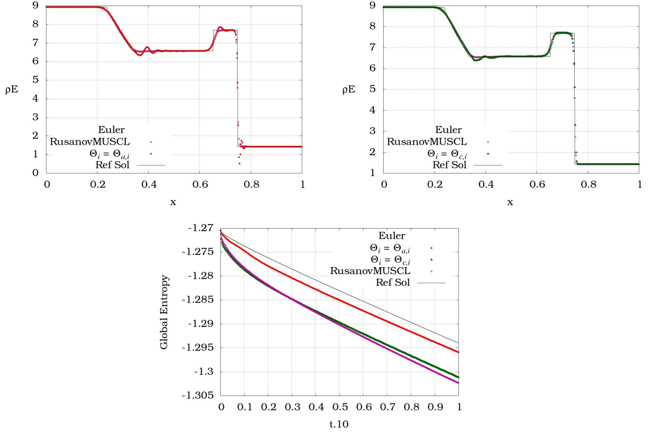
FIGURE 5. Second-order accurate approximation of the Euler solution for the Lax shock tube problem at time t = 0.1 with a mesh made of 400 cells: on the top wave profiles, on the bottom the decrease of the global entropy.
