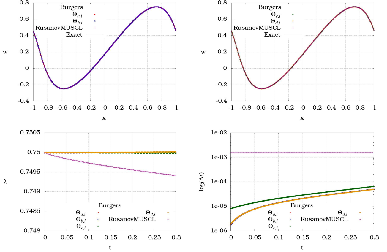
FIGURE 1. On the top, second-order accurate approximations of the smooth Burgers solutions at time t = 0.3 with a mesh made of 400 cells and with the \Theta_i^n matrices given by (5.1). On the bottom, comparison between (\lambda, \Delta t) given by our results (4.6)-(4.8) and the standard parameters used for the Rusanov MUSCL scheme endowed with the minmod slope limiter.
