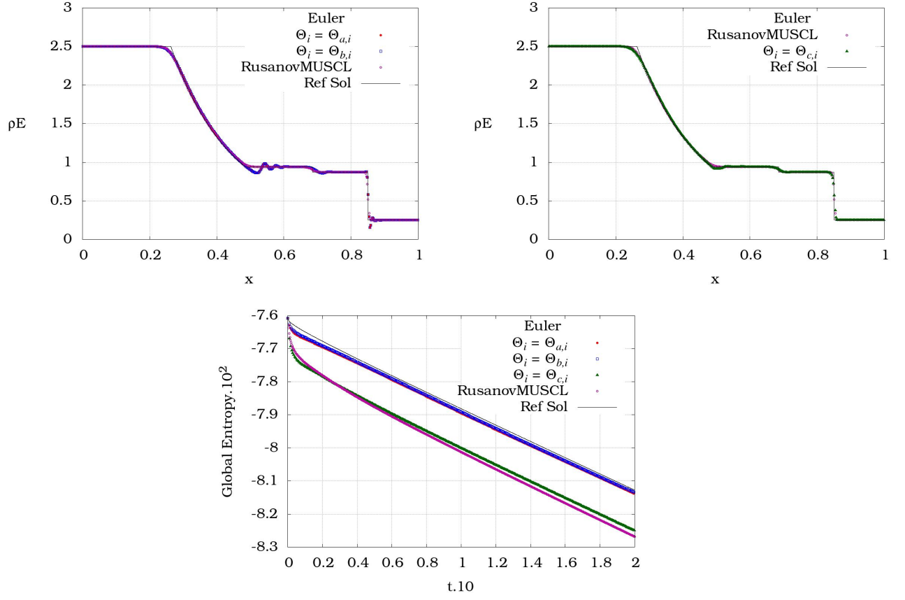
FIGURE 4. On the top, second-order accurate approximation of the Euler solution for the Sod shock tube problem at time t = 0.2 with a mesh made of 400 cells. On the bottom, the decrease of the global entropy integrated over the grid.
