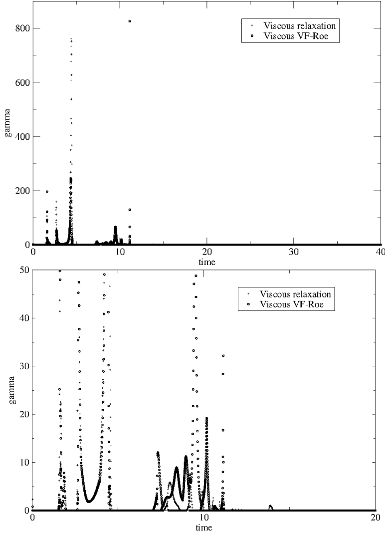
Fig. 7 Evolution of \gamma^n versus time (left) and a zoom (right) obtained for the subcritical flow at time t = 100 with 200 cells.
