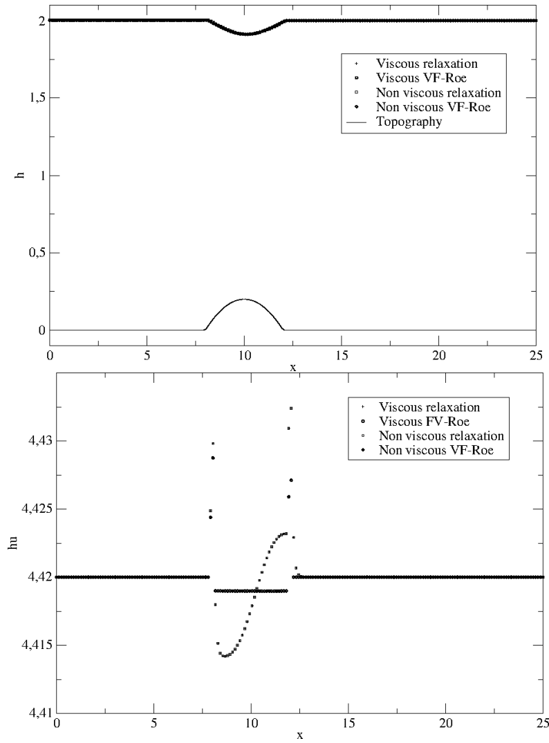
Fig. 6 Numerical simulation obtained for the subcritical flow at time t = 100 with 200 cells.
