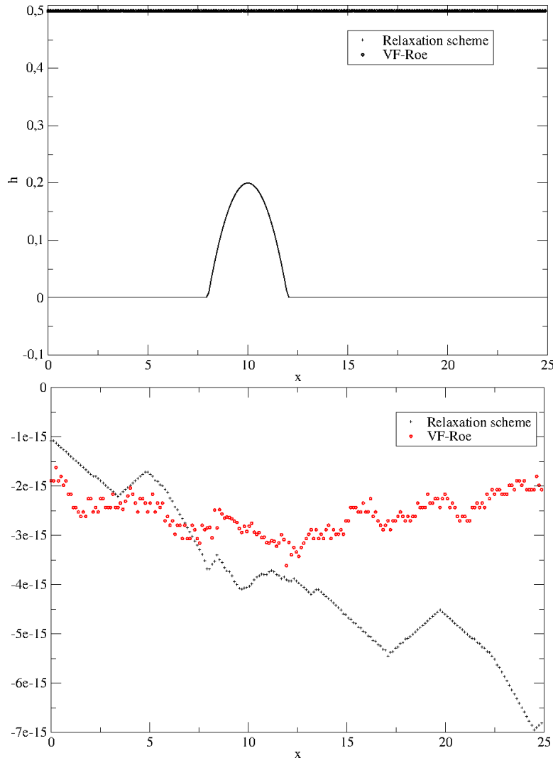
Fig. 5 Numerical simulation obtained for the lake at rest given for the initial data (53) at time t = 100 with 200 cells.
