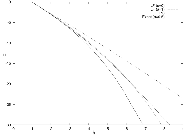
Figure 6: Hugoniot curves for a 1-shock in the Exner-Nielsen model: results for the HLL scheme with 2 definitions of \bar{h} , the Path-Consistent scheme and the exact solution with \alpha = 0.5
