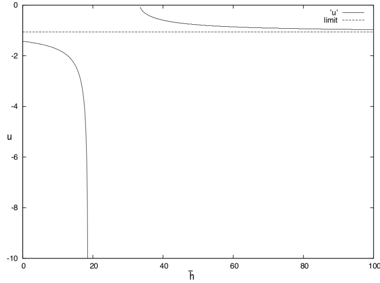
Figure 2: Hugoniot curves for a 1-shock in the Exner-Nielsen model: u as a function of \bar{h} and the limit value -\sqrt{\tau_c h^{1/3}} .
