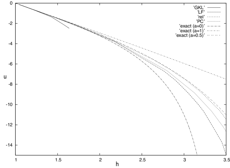
Figure 4: Hugoniot curves for a 1-shock in the Exner-Grass model: \alpha \in [0, 1] compared with the curves obtained by the four numerical schemes.
