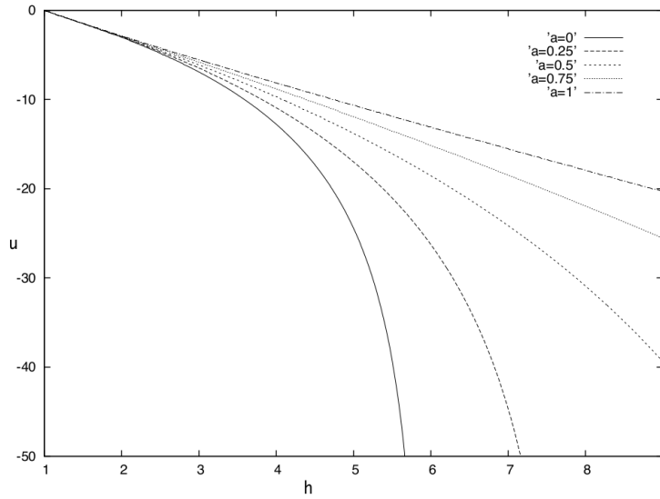
Figure 3: Hugoniot curves for a 1-shock in the Exner-Nielsen model: u as a function of h with the choice \bar{h} = \alpha h_L + (1 - \alpha)h for \alpha (bottom to top) 0, 0.25, 0.5, 0.75 and 1.
