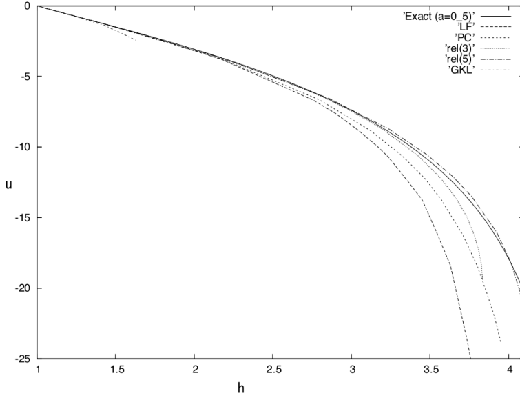
Figure 5: Hugoniot curves for a 1-shock in the Exner-Grass model: \alpha = \frac{1}{2} with the curves obtained by the numerical schemes.
