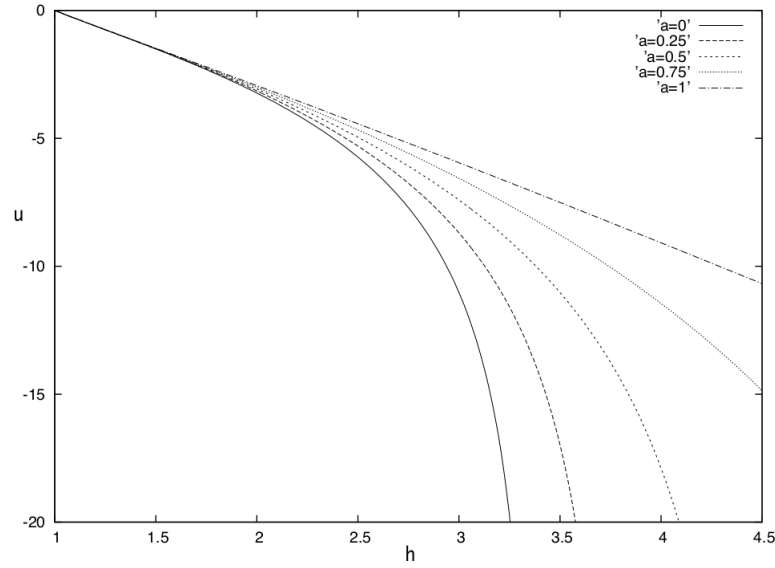
Figure 1: Hugoniot curves from the left state W_L = (1, 0, 1)^\top for a 1-shock in the Exner-Grass model: u as a function of h with \bar{h} = \alpha h_L + (1 - \alpha)h for \alpha \in [0, 1] .
