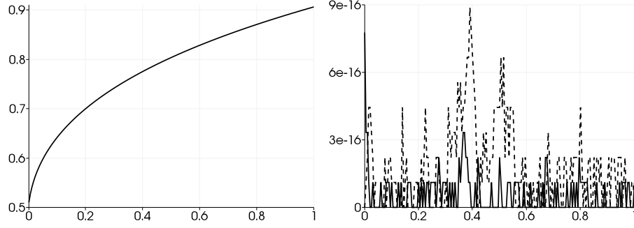
Figure 4: Left panel: initial height for the friction steady state. Right panel: height (solid line) and discharge (dashed line) errors to the steady state after 1s, with the explicit scheme.
