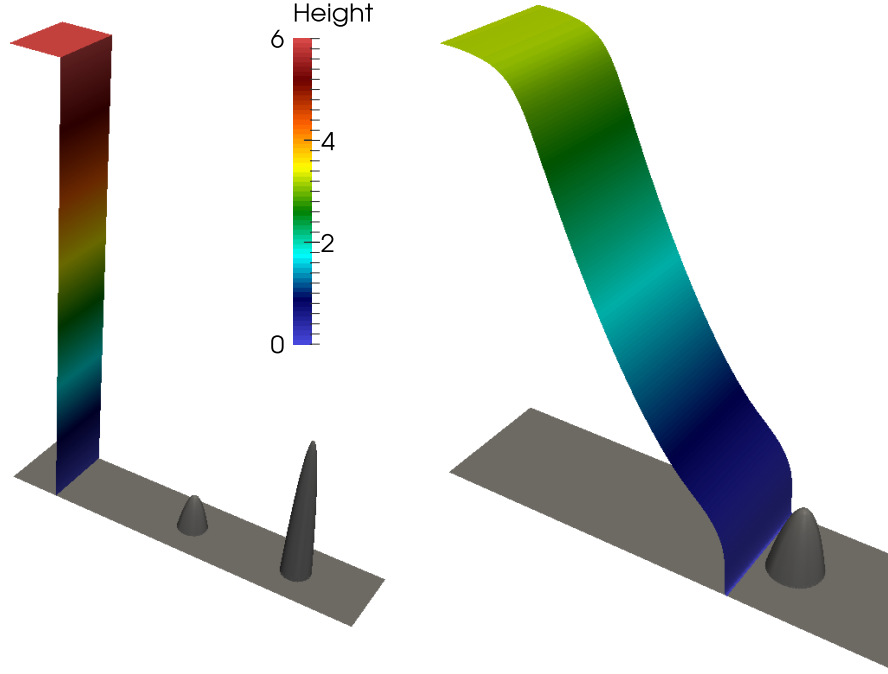
Figure 17: Left panel: initial condition of the 2D dam-break over a double bump experiment. Note that the same color scale for the water height is used in Figure 17 and Figure 18, and the solid gray color represents the topography. Right panel: approximate solution at t = 0.15 s, just before the water hits the first bump. Note the shape of the front of the water, due to the nonzero bottom friction.
