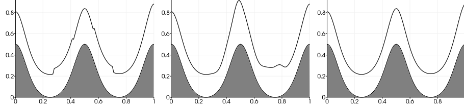
Figure 7: From left to right: water height for t = 0s , t = 0.015s and t = 2s , with the explicit scheme.
