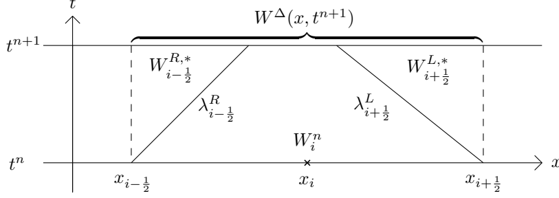
Figure 3: The full Godunov-type scheme using an approximate Riemann solver.
