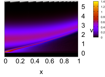
Ionic distribution - \nu=0.2 , \varepsilon^{\min}=0.63 , \alpha=0.9
