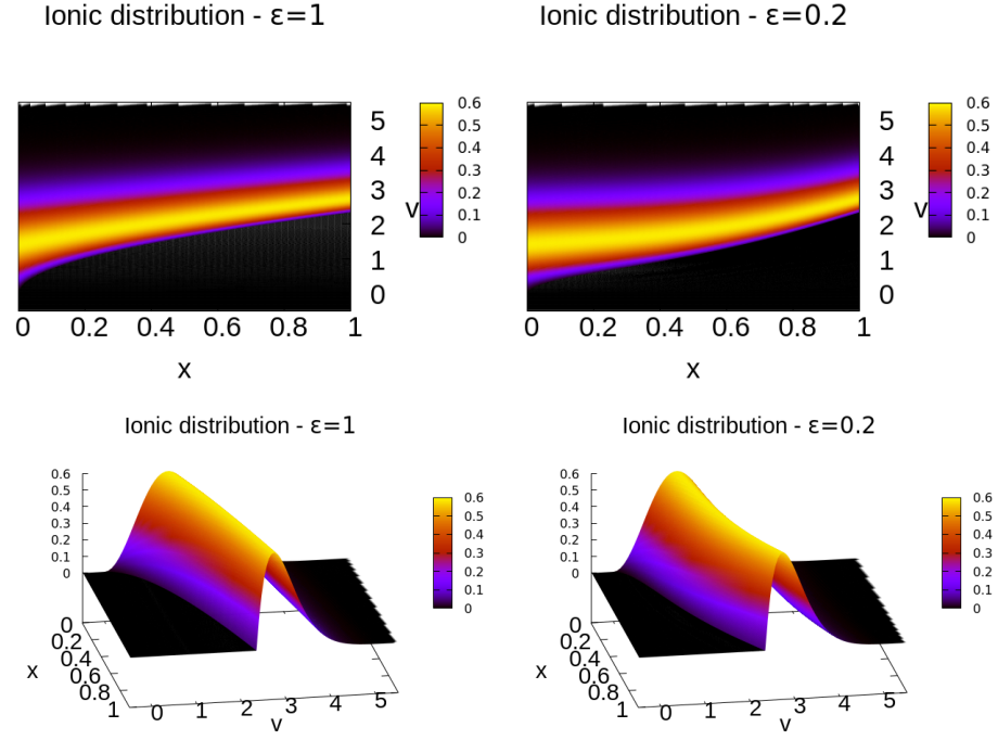
Figure 4: Ionic distribution function f_i(x, v) for two values of \varepsilon : 1 (left) and 0.2 (right), in the non collisional regime \nu = 0 , \alpha = 0 . Two different views on top and bottom.
