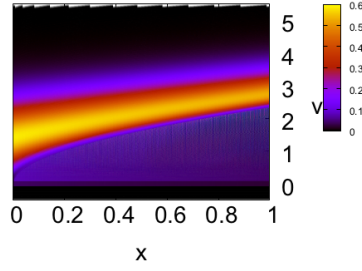
Ionic distribution - \nu=0.2 , \varepsilon=1 , \alpha=0.9
