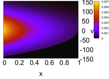
Electronic distribution - \nu=3.5, \varepsilon=1, \alpha=0
