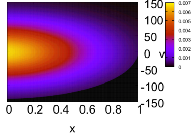
Electronic distribution - \nu=3.5, \varepsilon^{\min}=0.81, \alpha=0
