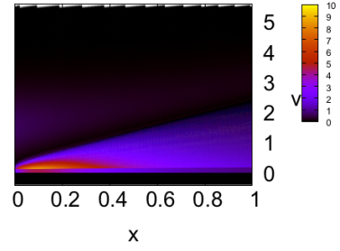
Figure 8: Ionic distribution function f_i(x, v) for \alpha = 0 , two values of \nu : 1 and 3.5 (from top to bottom). On the left: \varepsilon = 1 , on the right: \varepsilon = \varepsilon^{\min} .
