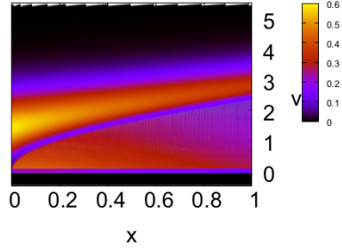
Ionic distribution - \nu=3.5 , \varepsilon=1 , \alpha=0
