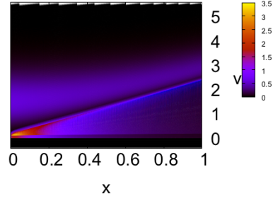
Ionic distribution - \nu=3.5 , \varepsilon^{\min}=0.81 , \alpha=0
