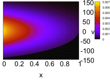
Figure 9: Electronic distribution function f_e(x, v) for \alpha = 0 , two values of \nu : 1 and 3.5 (from top to bottom). On the left: \varepsilon = 1 , on the right: \varepsilon = \varepsilon^{\min} .
