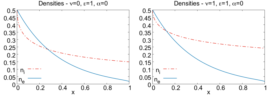
Figure 15: Ionic n_i(x) and electronic n_e(x) densities for \alpha = 0 , two values of \nu : 0 (on the left) and 1 (on the right).
