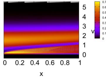
Figure 12: Ionic distribution function f_i(x, v) for \nu = 0.2 , two values of \alpha : 0 and 0.9 (from top to bottom). On the left: \varepsilon = 1 , on the right: \varepsilon = \varepsilon^{\min} .
