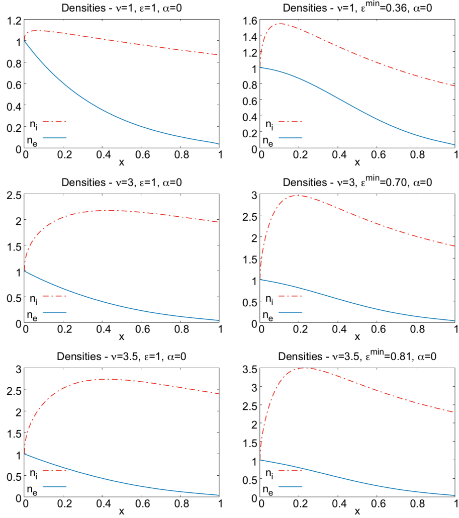
Figure 7: Ionic n_i(x) and electronic n_e(x) densities for \alpha = 0 , three values of \nu : 1, 3 and 3.5 (from top to bottom). On the left: \epsilon = 1 , on the right: \epsilon = \epsilon^{\min} .
