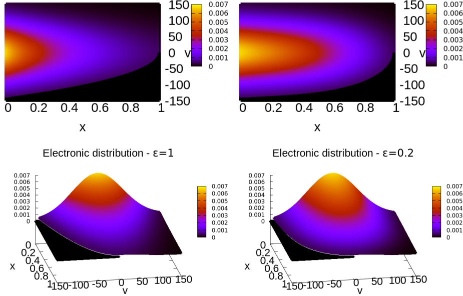
Electronic distribution - \varepsilon=1
