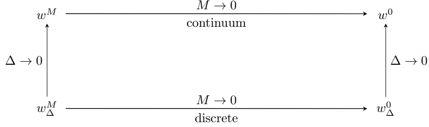
Figure 1: Asymptotic Preserving Diagram: w^M is a solution of system (2)-(3) and w^0 is a solution to (7) and w_\Delta^M and w_\Delta^0 are discrete approximations to the respective solutions.
