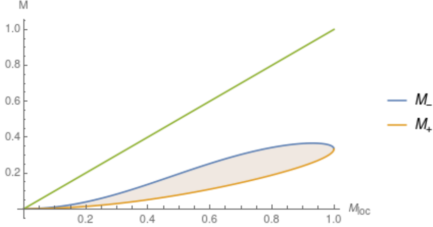
Figure 3: Functions M_{\pm} defined in (47). The green line gives the case M = M_{loc} for reference. The condition (47) states that the pair (M_{loc}, M) is not inside area between the curves M_{\pm} .
