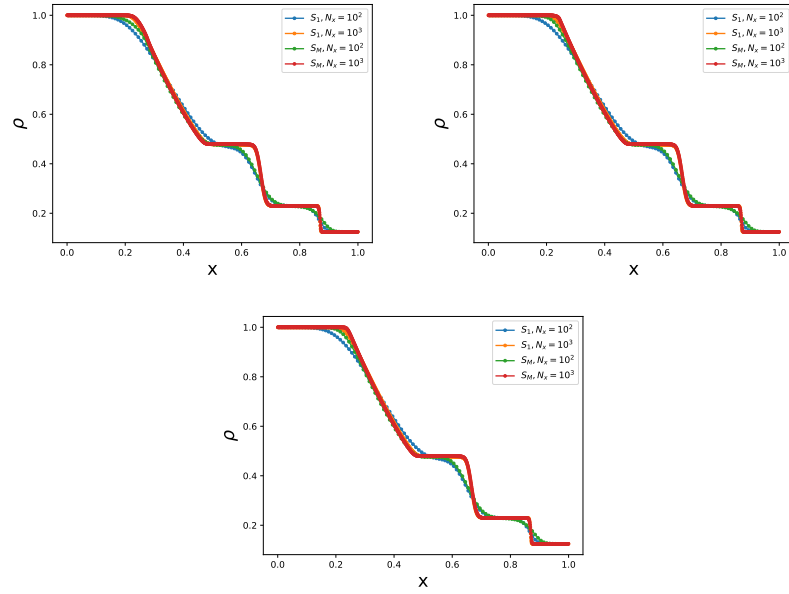
Figure 4: Numerical approximations to the Sod shock tube test for the schemes S_1 and S_M at different Mach numbers and at different resolutions at time 0.2. Top left: M = 10^{-1} . Top right: M = 10^{-2} . Bottom center: M = 10^{-3} .
