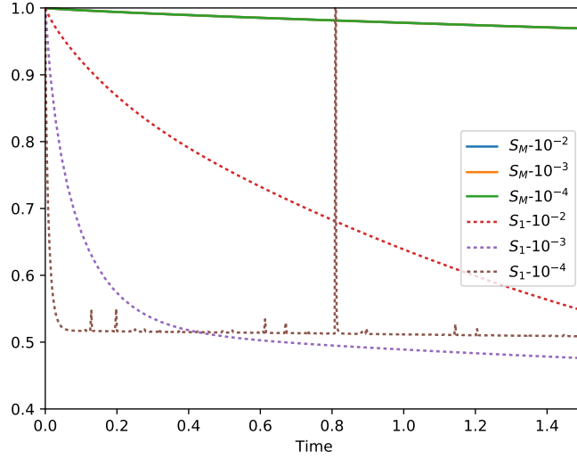
Figure 6: Evolution of the total kinetic energies in the numerical approximation of the Gresho vortex at different Mach numbers for different schemes. Shown is the relative total kinetic energy, i.e. \frac{tKE(t)}{tKE(0)} .
