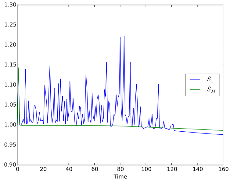
Figure 9: Kelvin-Helmholtz Instability: Evolution of the normed total kinetic energy for the schemes S_1 and S_M on a 128 \times 128 grid.
