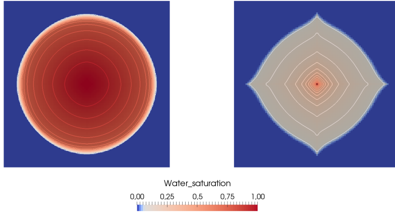
Figure 1: Grid orientation effect. Left: M = 0.8 ; right: M = 200 .
