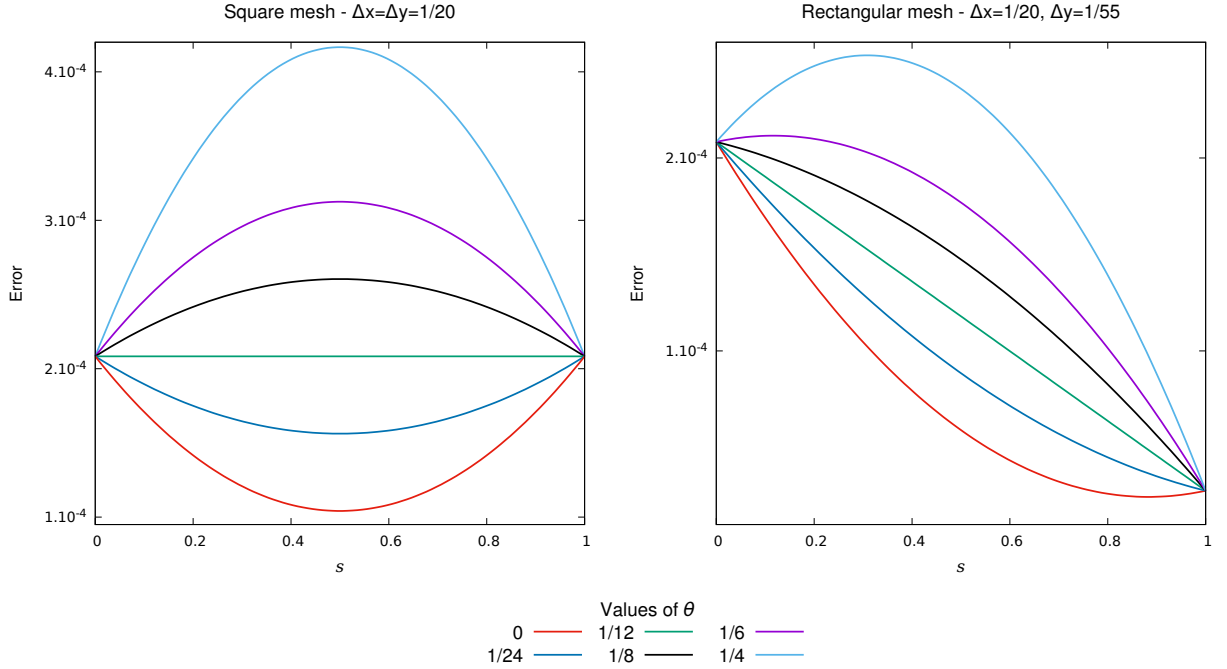
Figure 3: Angular error associated with the nine-point scheme S \mapsto \widetilde{\mathcal{E}}_{\Delta x, \Delta y}^{\theta}(S) for various \theta .
