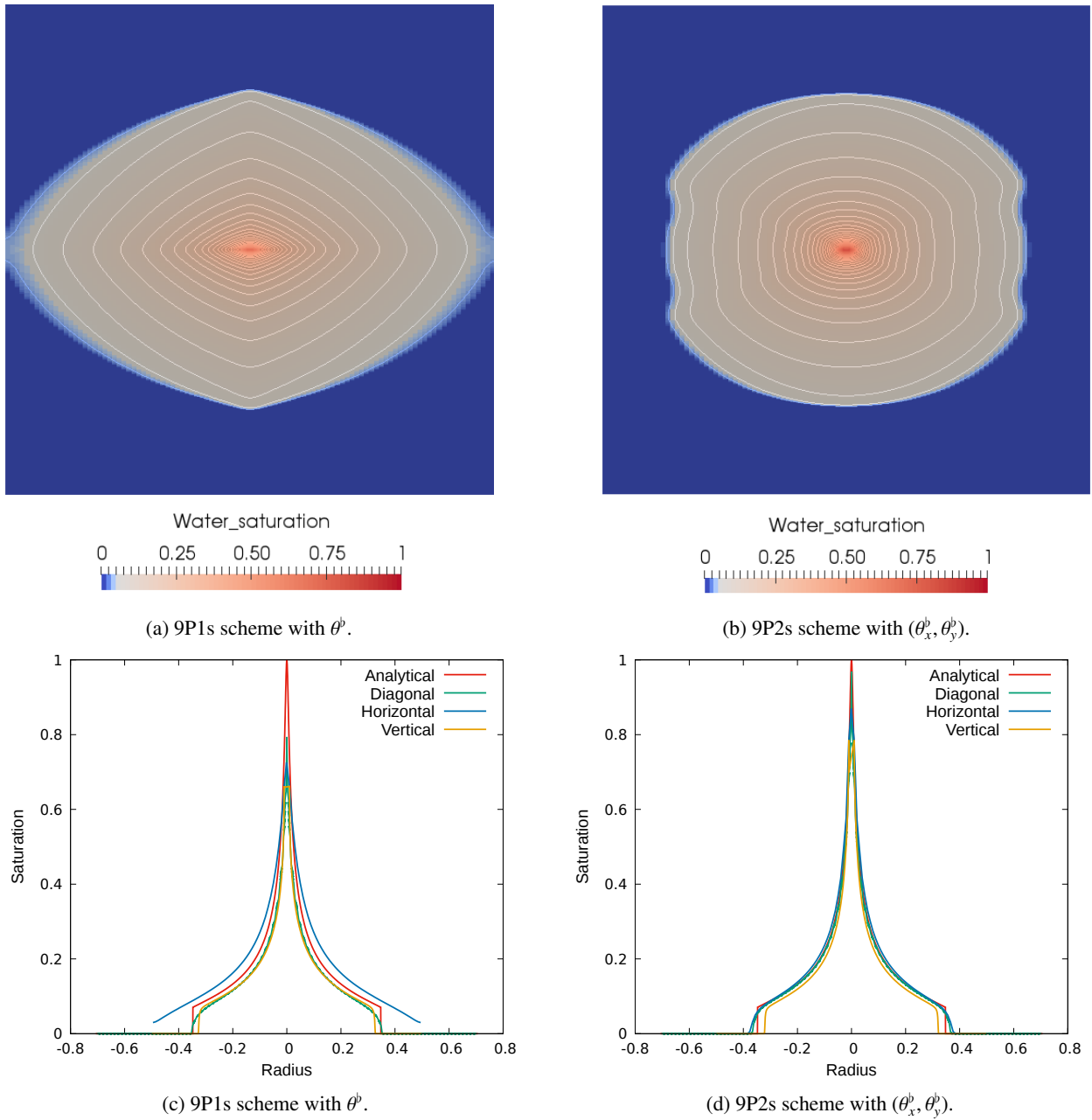
Figure 11: Water saturation fields (upper panels) and profiles (lower panels) for the radial problem on rectangular mesh ( \Delta x = 10\Delta y ) along the diagonal (green), horizontal (blue) and vertical (yellow) axes. Panel (a): \theta^b = 0.023635 . Panel (b): (\theta_x^b, \theta_y^b) = (0.243472, 0.069563) .
