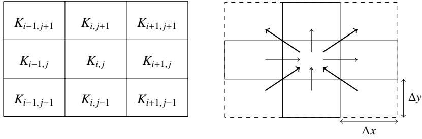
Figure 2: Nine-point stencil (left) and orientation of numerical fluxes (right).
