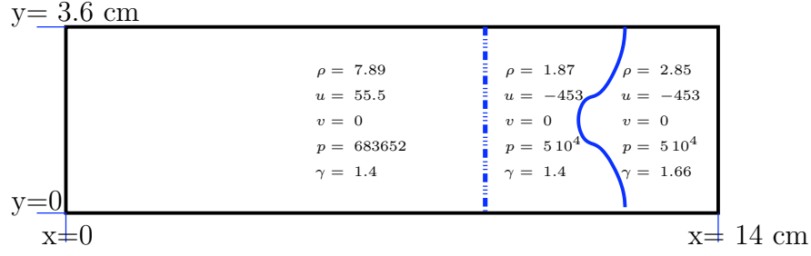
Fig. 1. Initialization of the non fluctuating variables.
