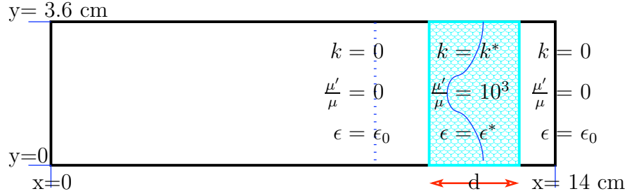
Fig. 2. Initialization of the fluctuating variables.
