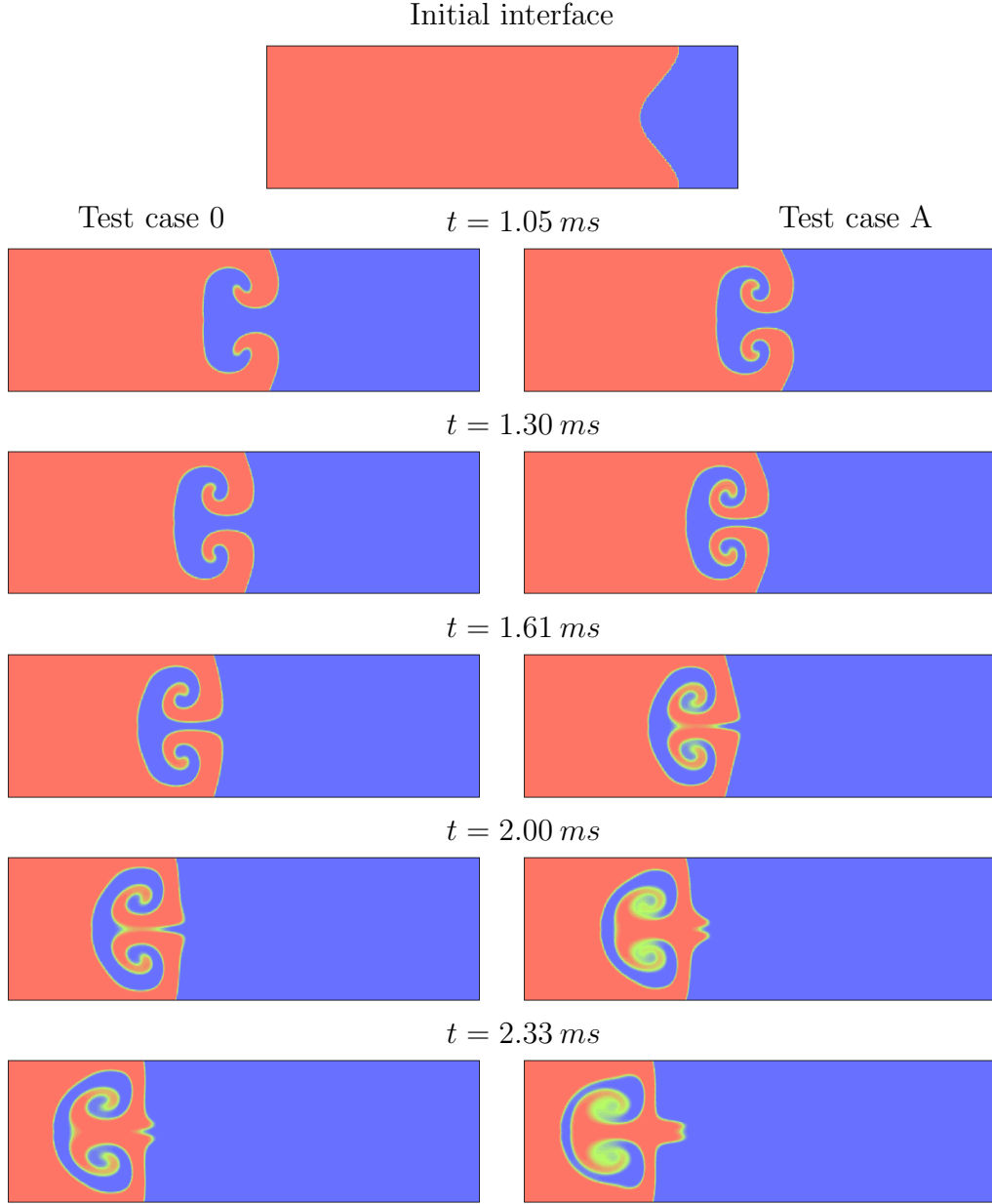
Fig. 3. Influence of the fluctuations on the behavior of the Richtmyer-Meshkov instability. Time evolution of a color function solution with (right) and without (left) an initial fluctuating zone around the material interface. Profiles (defined by the same color function) at the times t = 0 , t = 1.05 \text{ ms} , t = 1.3 \text{ ms} , t = 1.61 \text{ ms} , t = 2.0 \text{ ms} , t = 2.33 \text{ ms} .
