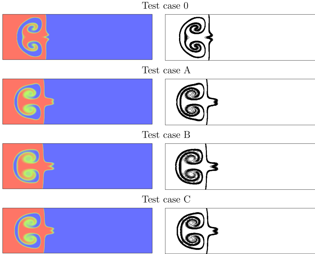
Fig. 5. Effects of the initial fluctuating conditions on the Richtmyer-Meshkov instability. Profiles (defined by the same color function) at the time t = 2.33 \text{ ms} .
