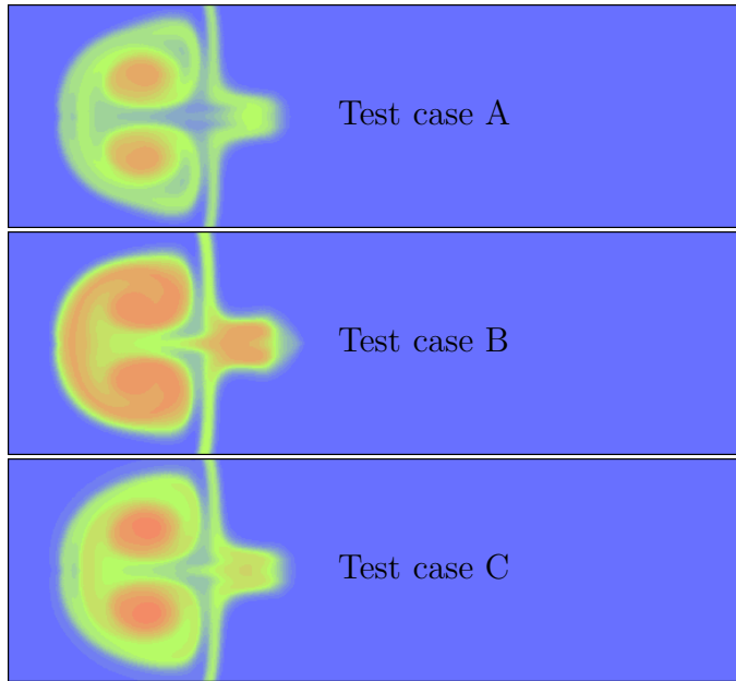
Fig. 6. Fluctuating kinetic energy \rho k at time t = 2.33 \text{ ms} . Profiles for the test cases A, B and C
