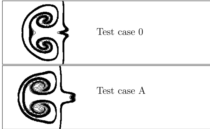
Fig. 4. Comparison of the numerical material interface profiles (defined by the same color function), at the time t = 2.33 \text{ ms} , between computations performed without (Test case 0) and with (Test case A) an initial fluctuating zone around the material interface.
