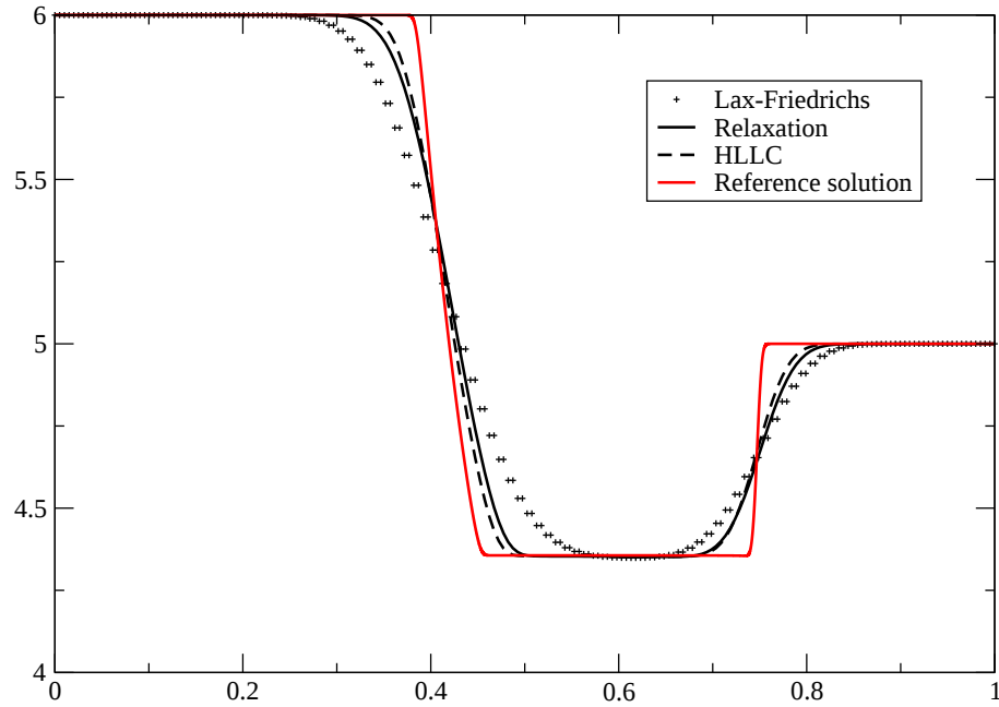
FIGURE 2.8 – Comparison between HLLC, Relaxation and Lax-Friedrichs' schemes.
