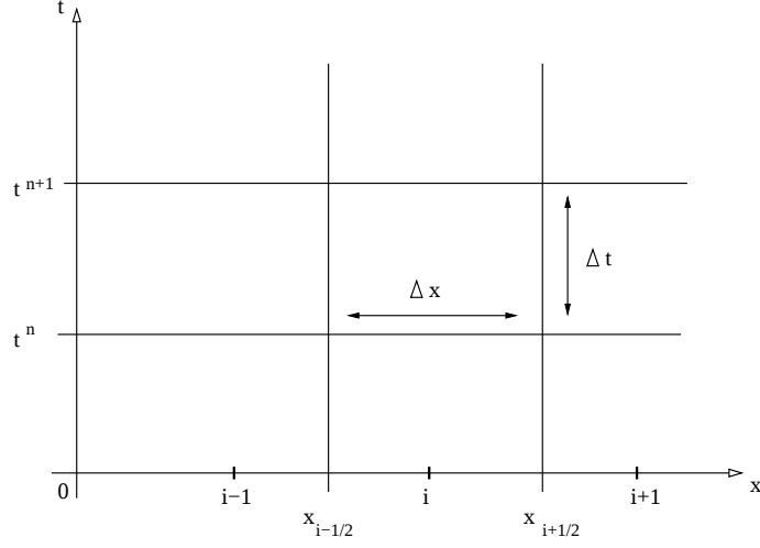
FIGURE 2.1 – Discretisation domain
