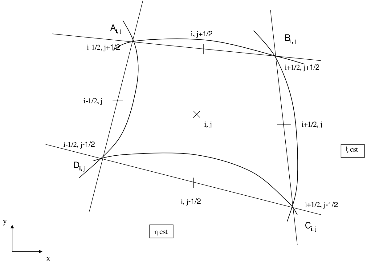
FIGURE 4.5 – Two dimensional curved grid
