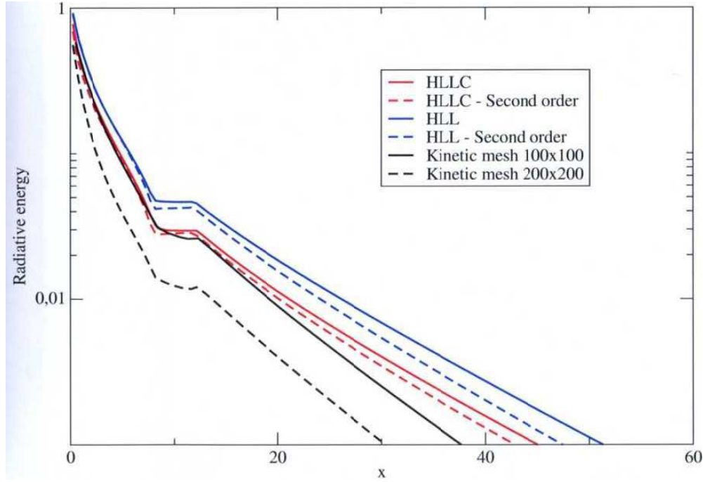
FIGURE 5.19 – Comparison of the radiative energy evolutions with a refined mesh.
