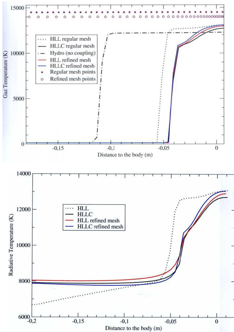
FIGURE 6.3 – Gas temperature (top) and radiative temperature (bottom) - Mesh convergence.
