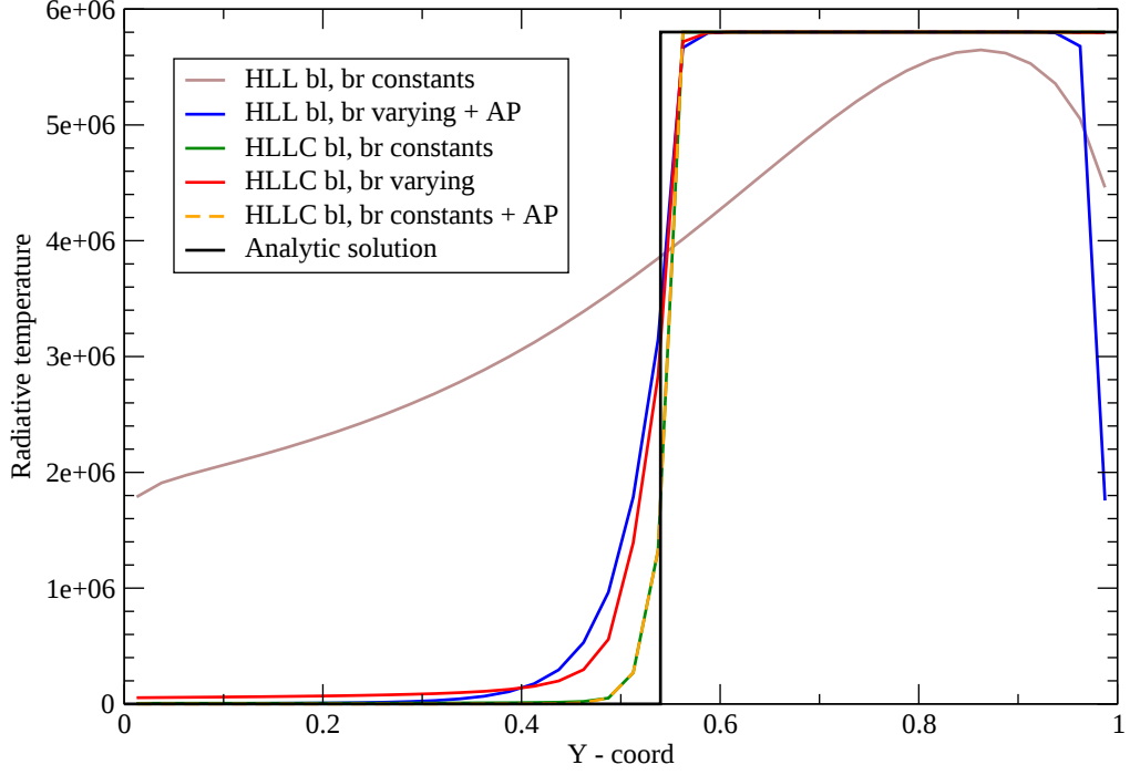
FIGURE 5.6 – Radiative temperature along the y coordinate.
