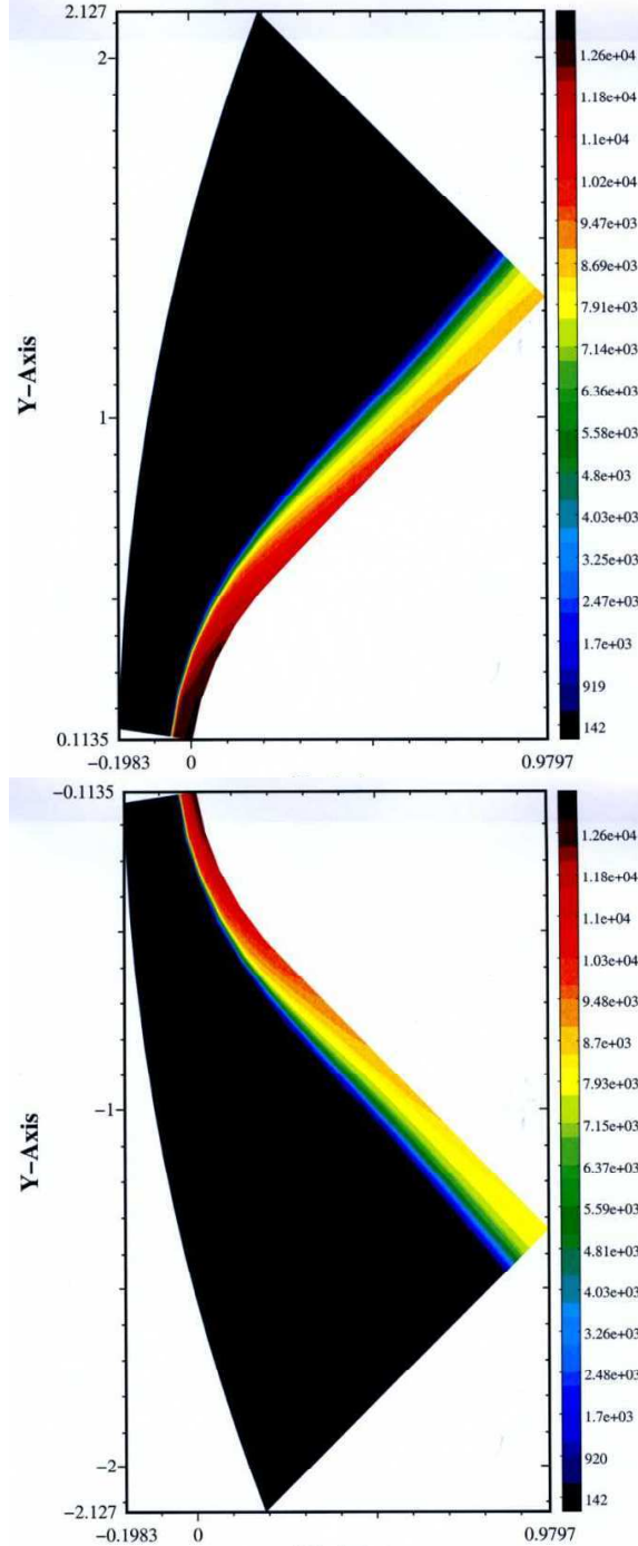
FIGURE 6.1 – Temperatures obtained the HLL (top) and HLLC (bottom) schemes.
