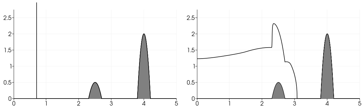
Figure 3.33 – Free surface for the double bump test case at different times. The gray area is the topography. Left panel: solution at t = 0\text{s} ; right panel: solution at t = 0.38\text{s} .
