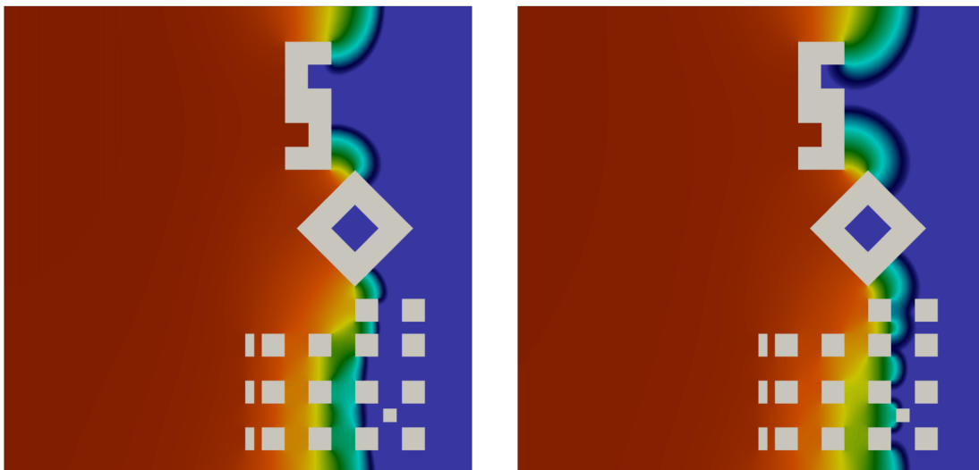
Figure 4.33 – Free surface for the urban topography simulation at t = 575\text{s} (left panel) and t = 630\text{s} (right panel).
