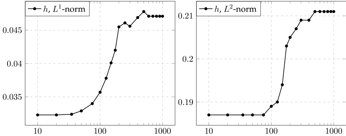
Figure 3.24 – Height error in L^1 -norm (left panel) and L^2 -norm (right panel) with respect to the parameter C .
