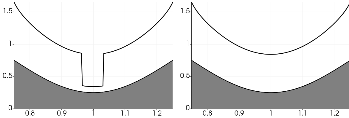
Figure 3.12 – Results of the explicit scheme. Left panel: free surface at t = 0\text{s} . Right panel: free surface at t = 3\text{s} .
