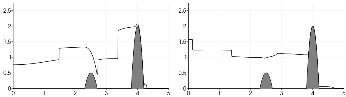
Figure 3.34 – Free surface for the double bump test case at different times. The gray area is the topography. Left panel: solution at t = 0.74\text{s} ; right panel: solution at t = 1.70\text{s} .
