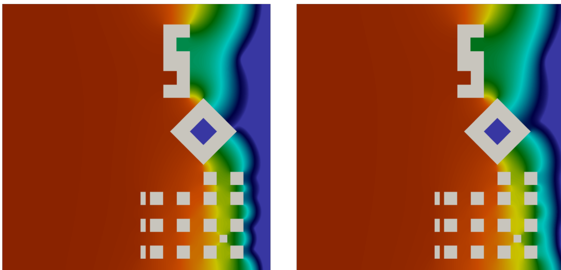
Figure 4.35 – Free surface for the urban topography simulation at t = 795\text{s} (left panel) and t = 850\text{s} (right panel).
