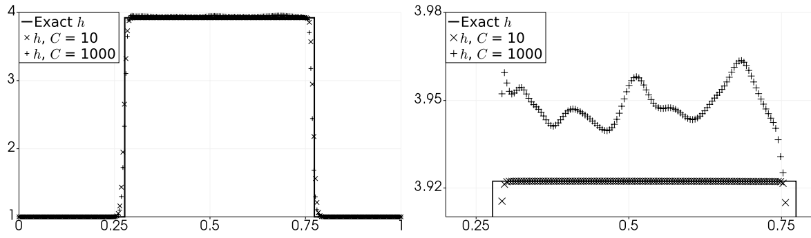
Figure 3.23 – Dam-break creating two shock waves over a flat bottom. Left panel: whole domain depicted at t = 0.1 s. Right panel: zoom on the intermediate state of the dam-break problem.
