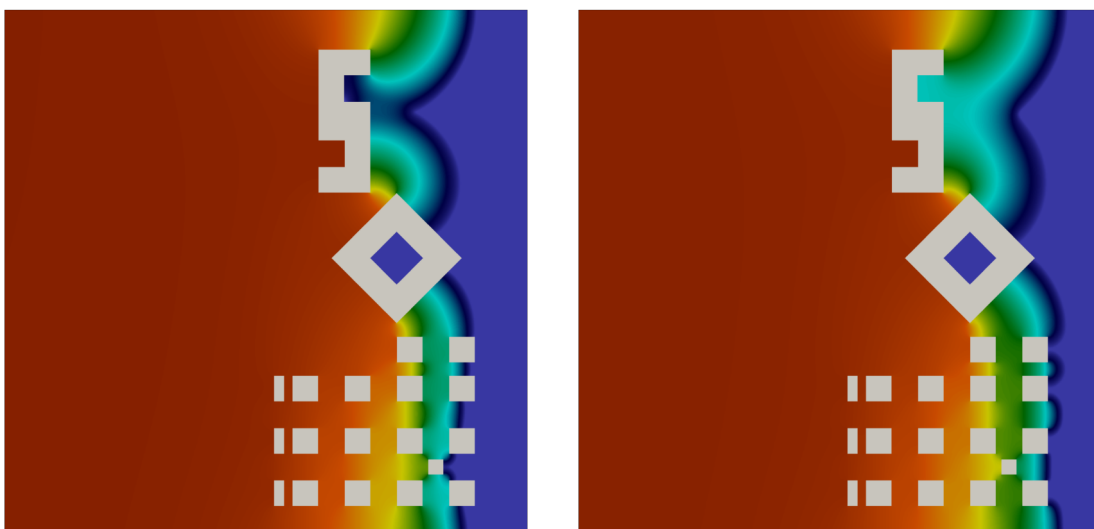
Figure 4.34 – Free surface for the urban topography simulation at t = 685\text{s} (left panel) and t = 740\text{s} (right panel).
